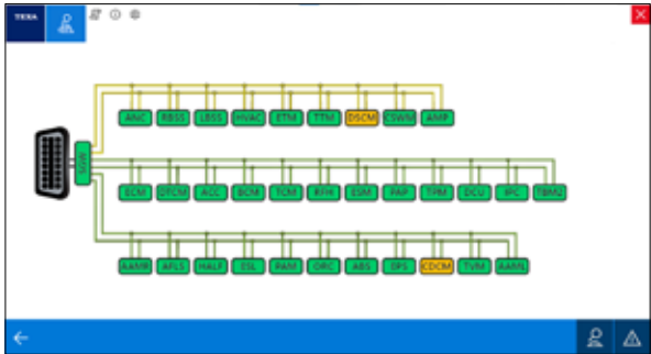
TGS3s DASHBOARDS.
